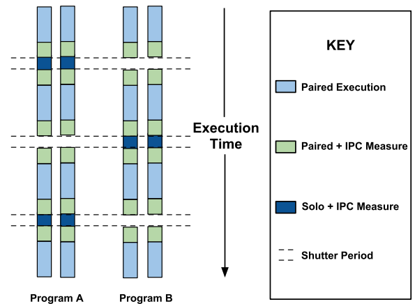
Fig. 3. Shown here is shuttering in action on two separate jobs. During a shutter, one job executes while all others sleep. (Colors are visible in the online version of the article; http://dx.doi.org/10.3233/SPR-140387 .)
