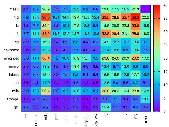
Fig. 11. Performance degradation (%) for jobs on the x -axis co-located with jobs on the y -axis. (Colors are visible in the online version of the article; http://dx.doi.org/10.3233/SPR-140387 .)
