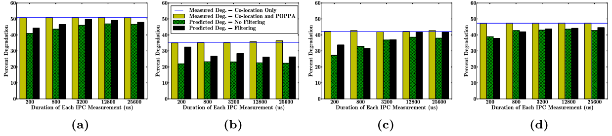
Fig. 6. Effect of shutter duration on accuracy and overhead for each NPB co-run with ADVECT3D-256. (a) CG. (b) FT. (c) LU. (d) MG. (Colors are visible in the online version of the article; http://dx.doi.org/10.3233/SPR-140387 .)
