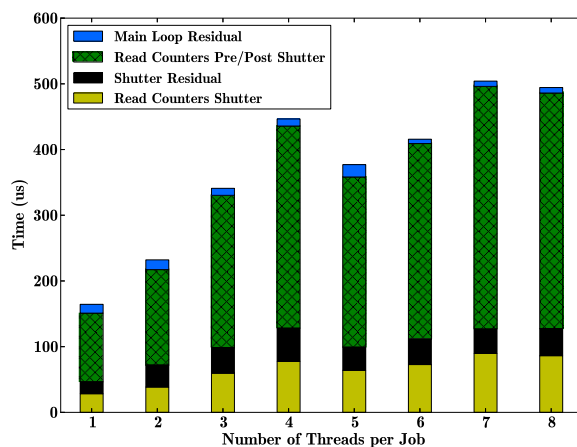
Fig. 4. Breakdown of base overhead to execute a single iteration of POPPA's core algorithm, where reading PMC values dominates total time. (Colors are visible in the online version of the article; http://dx.doi.org/10.3233/SPR-140387 .)
