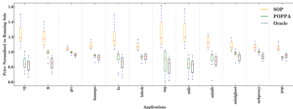
Fig. 12. The distribution of prices a user would pay for a given application when using either the state-of-practice (SOP), POPPA, or the maximally fair Oracle. (Colors are visible in the online version of the article; http://dx.doi.org/10.3233/SPR-140387 .)
