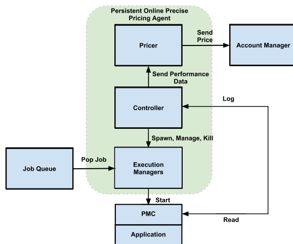
Fig. 2. Interaction between POPPA components and other entities. (Colors are visible in the online version of the article; http://dx.doi.org/10.3233/SPR-140387 .)
