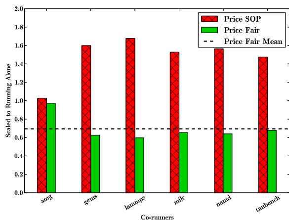
Fig. 1. Performance of GTC, a plasma physics code, when co-located with the applications on the x -axis. The current pricing mechanism penalizes the user for co-locating their job by charging them more when their job degrades more. (Colors are visible in the online version of the article; http://dx.doi.org/10.3233/SPR-140387 .)
