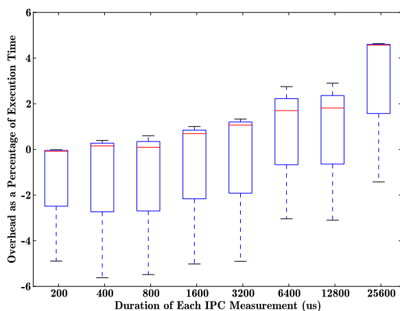
Fig. 9. Overhead of POPPA on NAS benchmarks co-located with Swim-150. (Colors are visible in the online version of the article; http://dx.doi.org/10.3233/SPR-140387 .)
