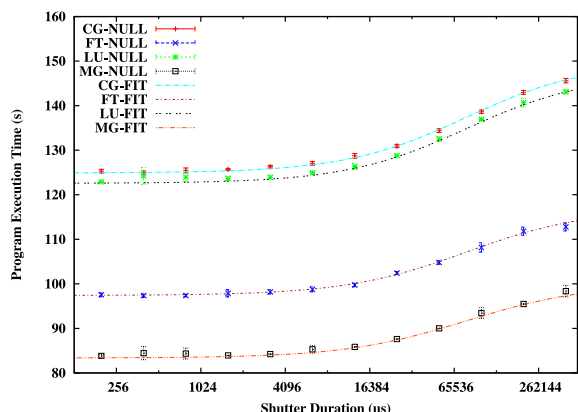
Fig. 5. The relative overhead of expanding the duration of a shutter, where points correspond to measurements and lines correspond to instantiations of the model. (Colors are visible in the online version of the article; http://dx.doi.org/10.3233/SPR-140387 .)
