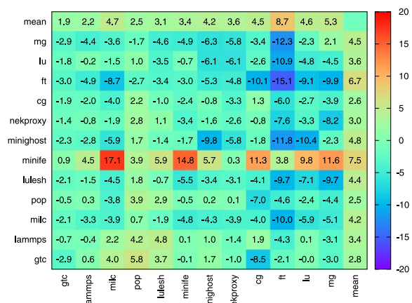
Fig. 10. Run time prediction accuracy (%) for jobs on the x -axis co-located with jobs on the y -axis. (Colors are visible in the online version of the article; http://dx.doi.org/10.3233/SPR-140387 .)
