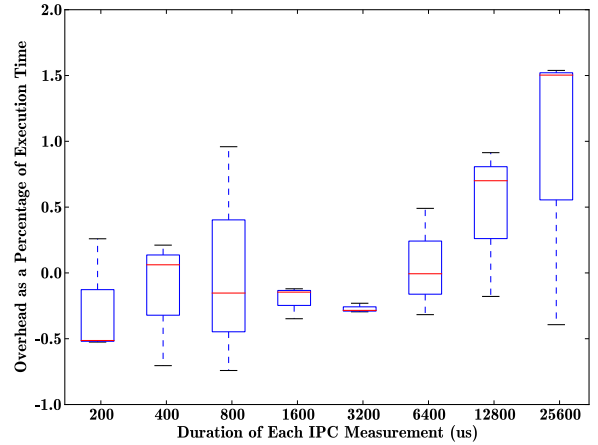
Fig. 8. Overhead of POPPA on NAS benchmarks co-located with ADVECT-256. (Colors are visible in the online version of the article; http://dx.doi.org/10.3233/SPR-140387 .)
