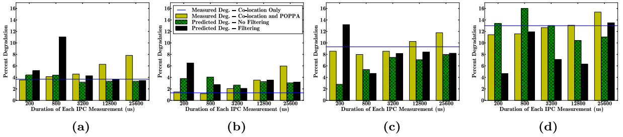
Fig. 7. Effect of shutter duration on accuracy and overhead for each NPB co-run with Swim-150. (a) CG. (b) FT. (c) LU. (d) MG. (Colors are visible in the online version of the article; http://dx.doi.org/10.3233/SPR-140387 .)
