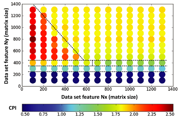
Fig. 10. CPI behavior of a matrix–matrix multiply benchmark on Intel i5 platform vs matrix size. Hyperplanes separate areas with similar behavior found using multivariate adaptive regression splines (MARS). (Colors are visible in the online version of the article; http://dx.doi.org/10.3233/SPR-140396 .)
