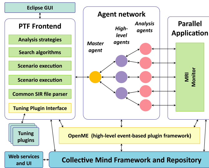
Fig. 12. PTF plugin-based application online tuning framework. (Colors are visible in the online version of the article; http://dx.doi.org/10.3233/SPR-140396 .)
