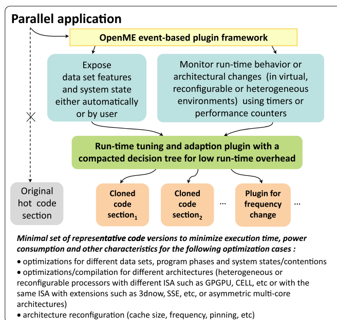
Fig. 13. Making run-time adaptation and tuning practical using static multi-versioning, features exposed by users or automatically detected, and predictive modeling (decision trees) while avoiding complex dynamic recompilation frameworks. (Colors are visible in the online version of the article; http://dx.doi.org/10.3233/SPR-140396 .)
