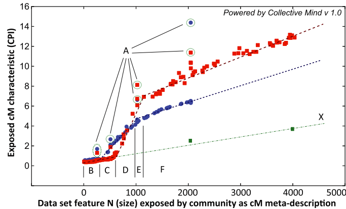
Fig. 9. Online learning (predictive modeling) of a CPI behavior of a shared LU-decomposition benchmark on 2 different platforms (Intel Core2 shown in red vs Intel i5 shown in blue) vs vector size N (data set feature). (Colors are visible in the online version of the article; http://dx.doi.org/10.3233/SPR-140396 .)
