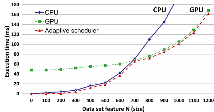
Fig. 3. Execution time of a matrix–matrix multiply kernel when executed on CPU (Intel E6600) and on GPU (NVIDIA 8600 GTS) depending on size N of square matrix as a motivation for online tuning and adaptive scheduling on heterogeneous architectures [46]. (Colors are visible in the online version of the article; http://dx.doi.org/10.3233/SPR-140396 .)
