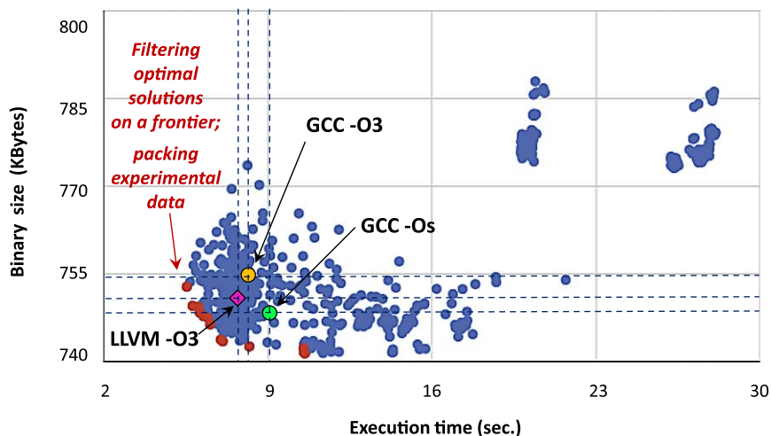
Fig. 8. Compiler flag auto-tuning to improve execution time and code size of a shared image corner detection program with a fixed data set on Samsung Galaxy Series mobile phone using cM for Android. Highlighted points represent frontier of optimal solutions as well as GCC with -O3 and -Os optimization flags versus LLVM with -O3 flag ( c-mind.org/interactive-graph-demo ). (Colors are visible in the online version of the article; http://dx.doi.org/10.3233/SPR-140396 .)
