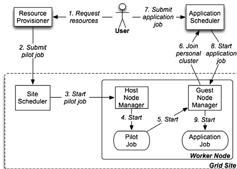
Fig. 1. Multi-level scheduling.
