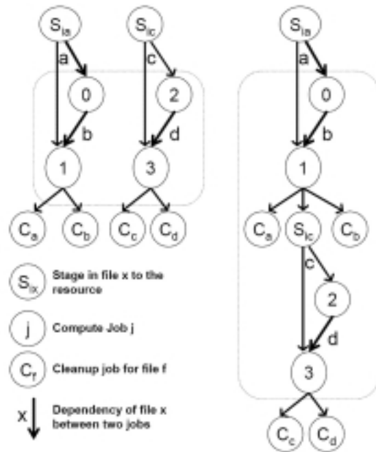
Fig. 12. An example workflow before and after restructuring.
