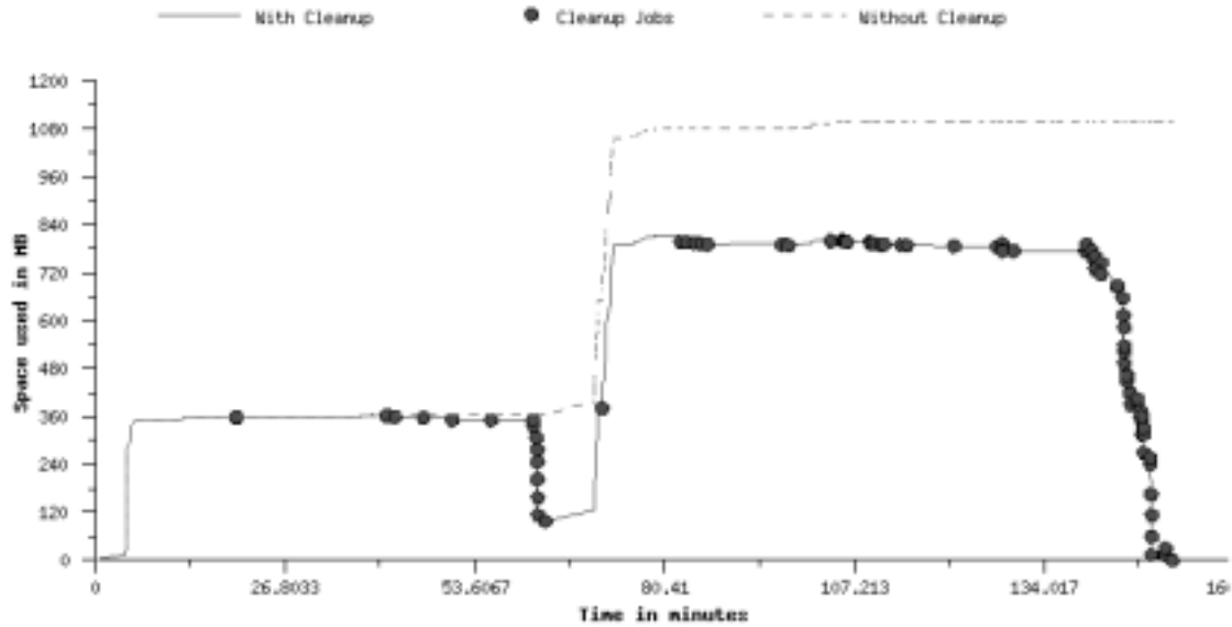
Fig. 16. Behavior of the moderately-restructured workflow on the OSG.
