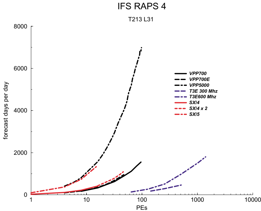
Fig. 1. IFS RAPS 4: T213L31. Courtesy of ECMWF and David Dent.
