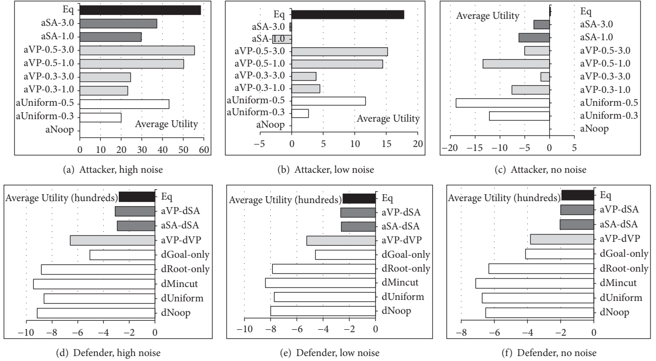
FIGURE 12: Strategy evaluation, random DAGs, 0% \Lambda -nodes.
