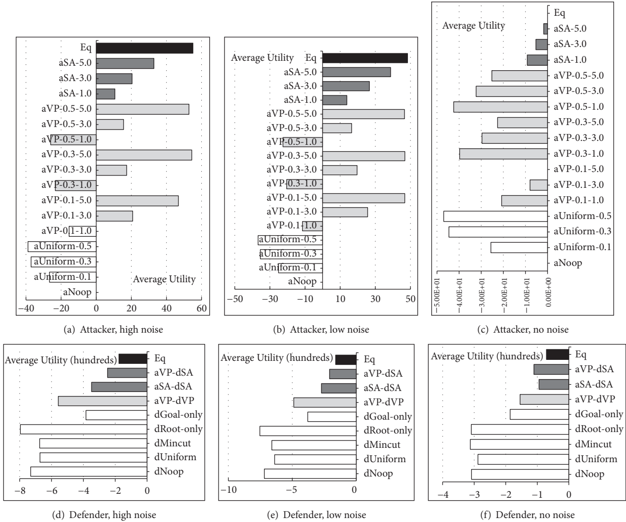
FIGURE 13: Robustness evaluation, layered DAGs, 0% \Lambda -nodes.
