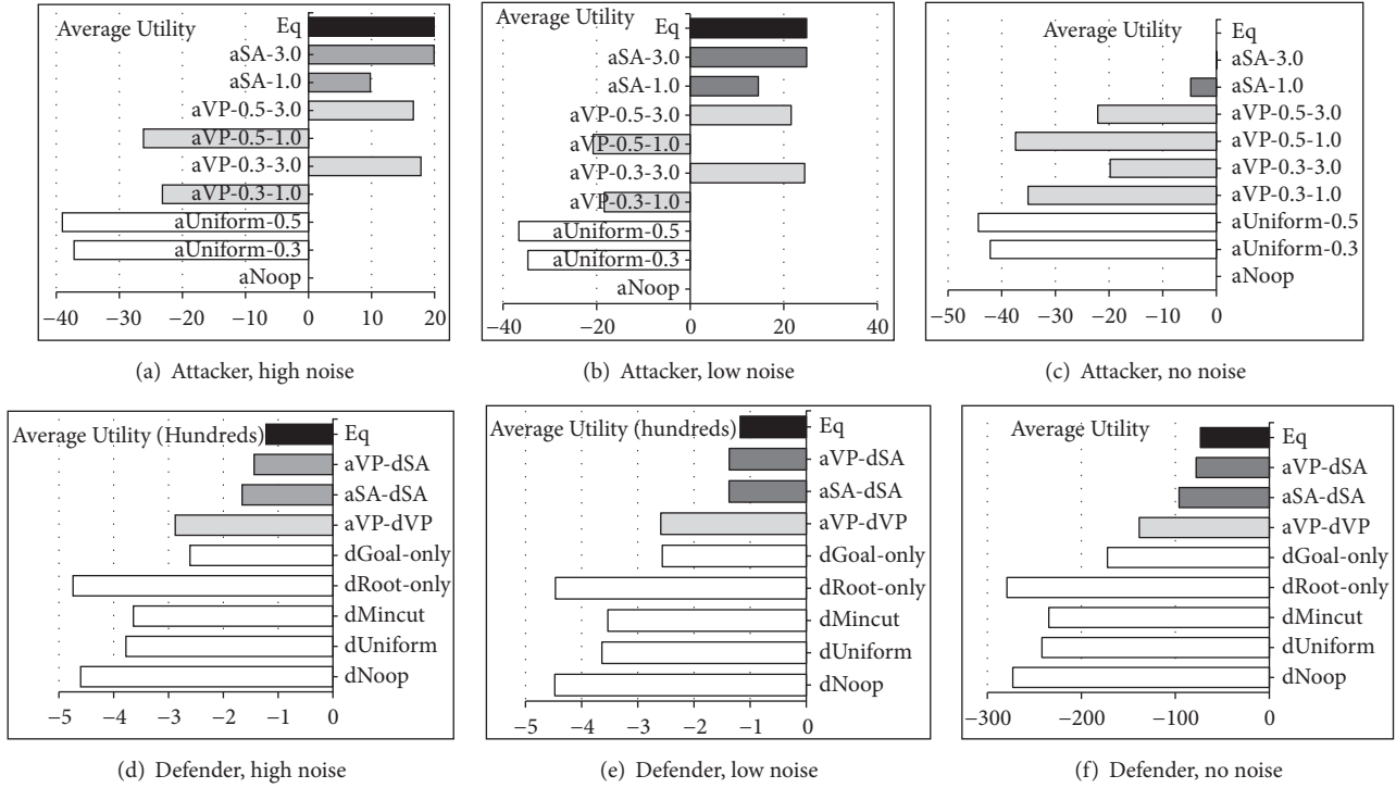
FIGURE 10: Strategy evaluation, layered DAGs, 0% \Lambda -nodes.
