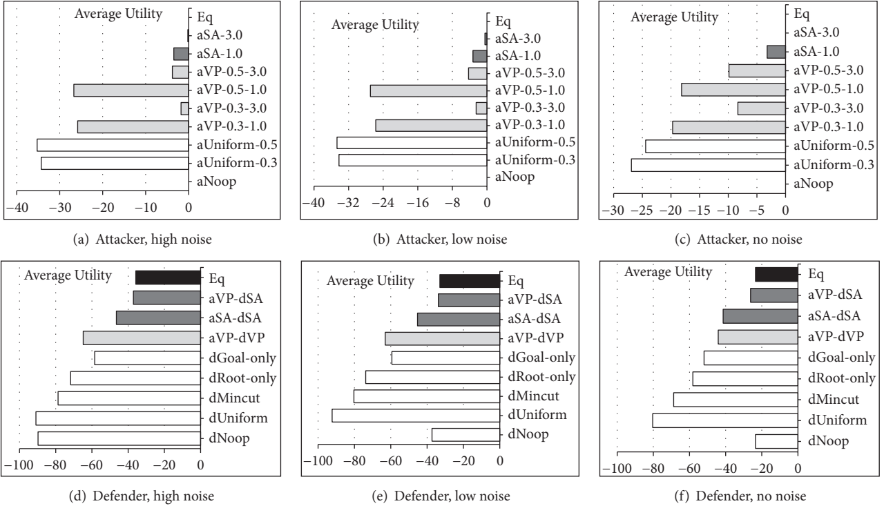
FIGURE 11: Strategy evaluation, layered DAGs, 50% \wedge -nodes.
