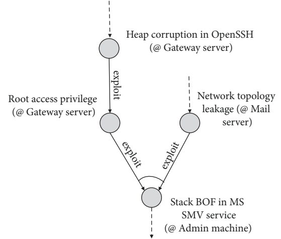
FIGURE 1: Portion of Bayesian attack graph for testbed network of Poolsappasit et al. [18]. The node with exploits connected by an arc is \wedge -type; the rest are \vee -type. Dotted edges indicate excluded portions of the graph. In this graph portion, there are four nodes representing system vulnerabilities and access privileges. The attacker can exploit the heap corruption in OpenSSH at the gateway server to obtain root access privileges. Then the attacker can exploit root access privileges at the gateway server and the network topology leakage at the mail server to cause the stack BOF in the MS SMV service of the admin machine.
