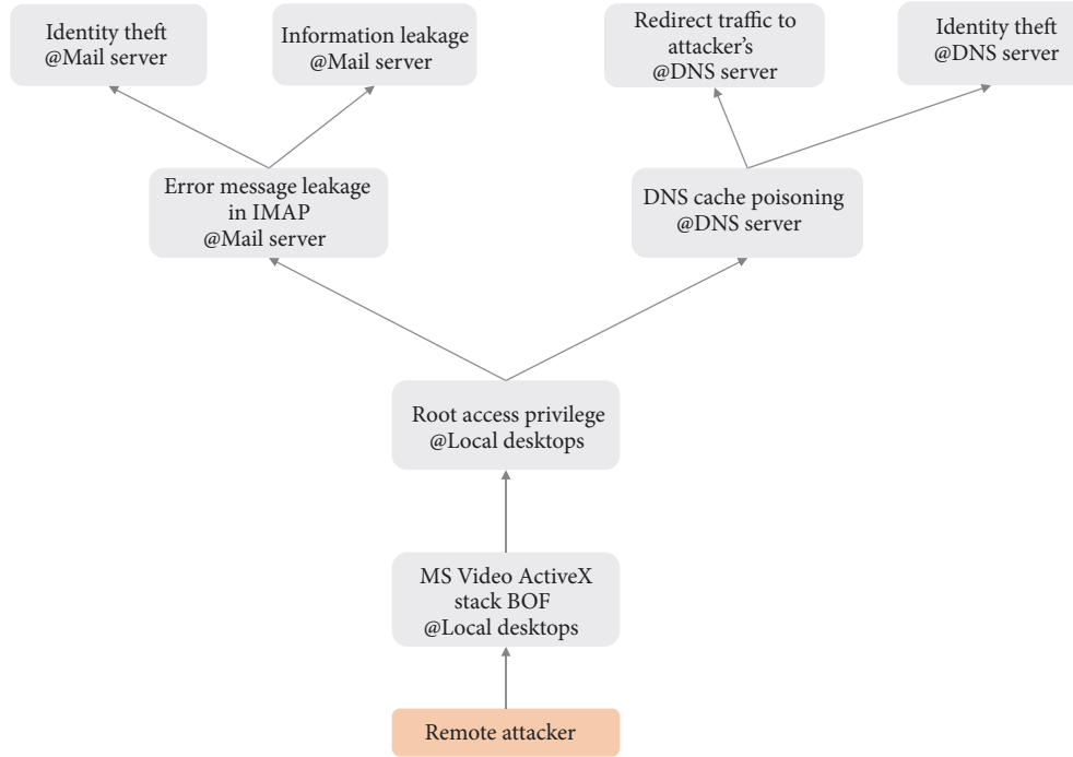
FIGURE 3: A portion of the Bayesian attack graph of the testbed network in Poolsappasit et al. [18].
