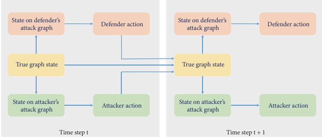
FIGURE 9: Empirical game-theoretic analysis simulation.
