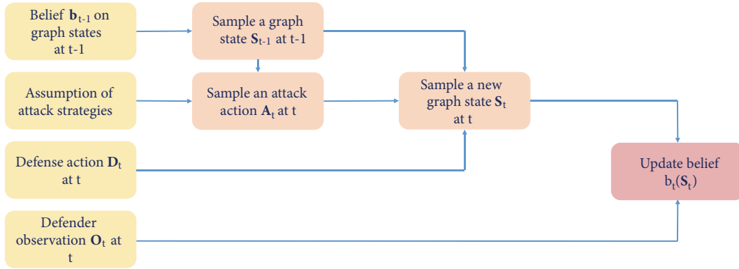
FIGURE 6: Overview of the defender belief update on graph states.
