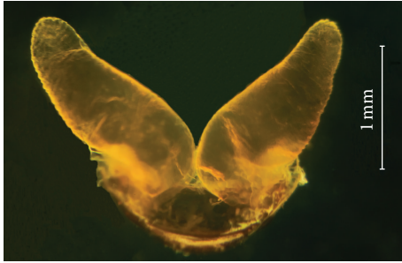
FIGURE 1: Defensive gland of Mesomorpha villiger cut from the remainder of the sternites.
