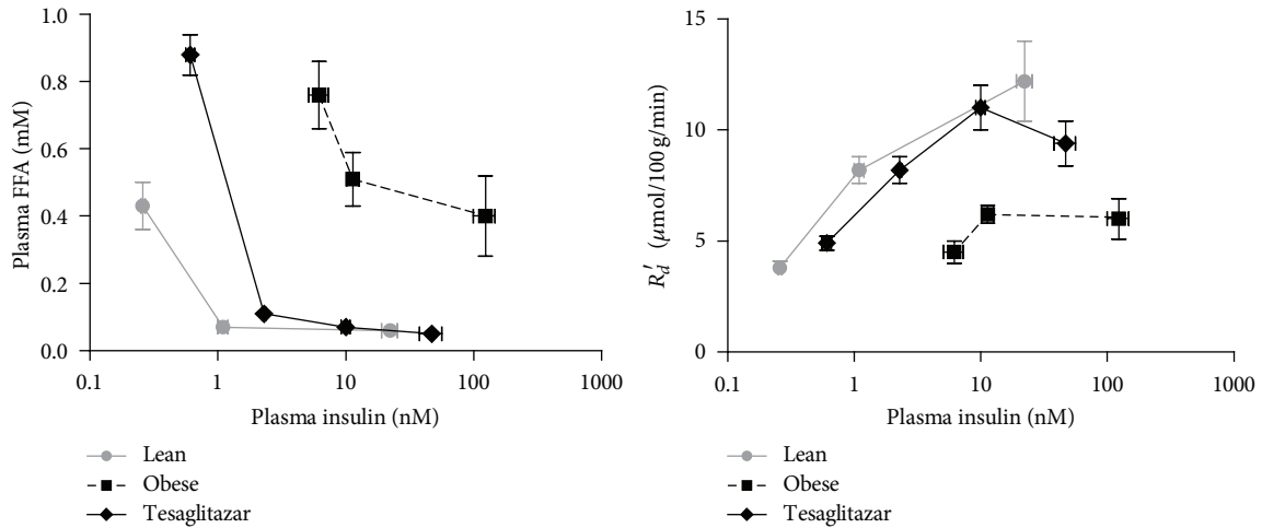
FIGURE 2: Whole body effects of insulin, under basal and hyperinsulinemic clamp conditions: suppression of plasma FFA and stimulation of glucose disposal rate R_d^i (=“average” tissue utilization rate) in Lean, Obese, and Tesaglitazar groups of Zucker rats. Data points represent means \pm SE ( n = 5-7 ).
