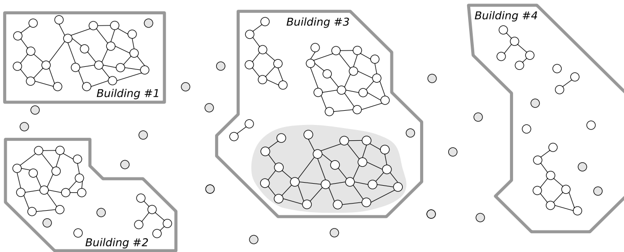
Fig. 1. Example of a disconnected MANET.
