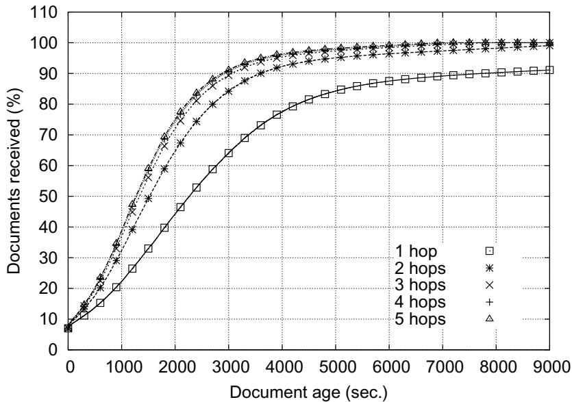
(b) Smoothed cumulative distribution of the age of documents at delivery-time
