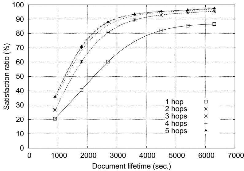
Fig. 19. Comparison of the MPR-based and flooding-based versions of the protocol.
