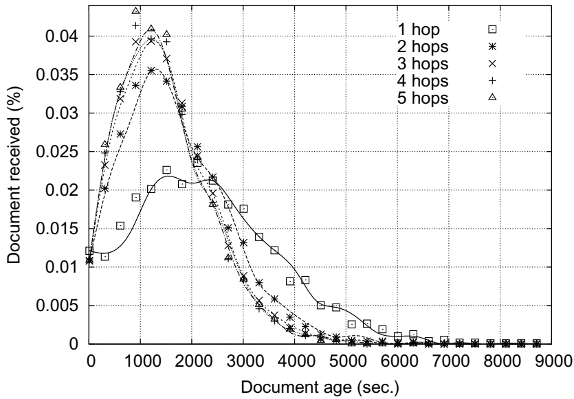
(a) Distribution of the age of documents at delivery-time
