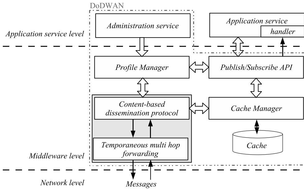
Fig. 3. Architecture of the communication platform.
