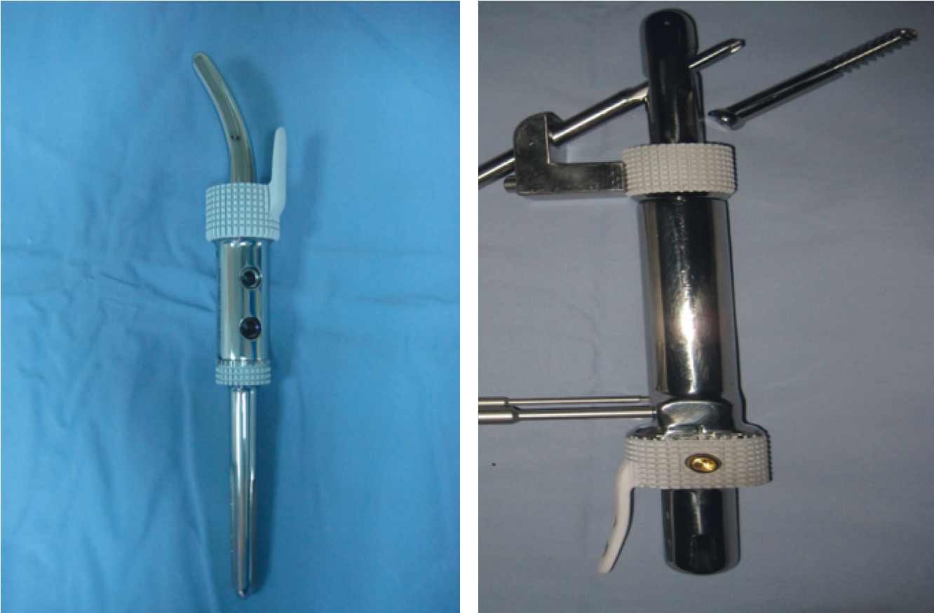
(a) (b) FIGURE 2: (a) Custom JSE with curved stem and HA-coated side plate suitable for proximal femur. (b) Custom JSE for proximal femur and distal femur with cross screw, and one side plate for the distal femur side.
