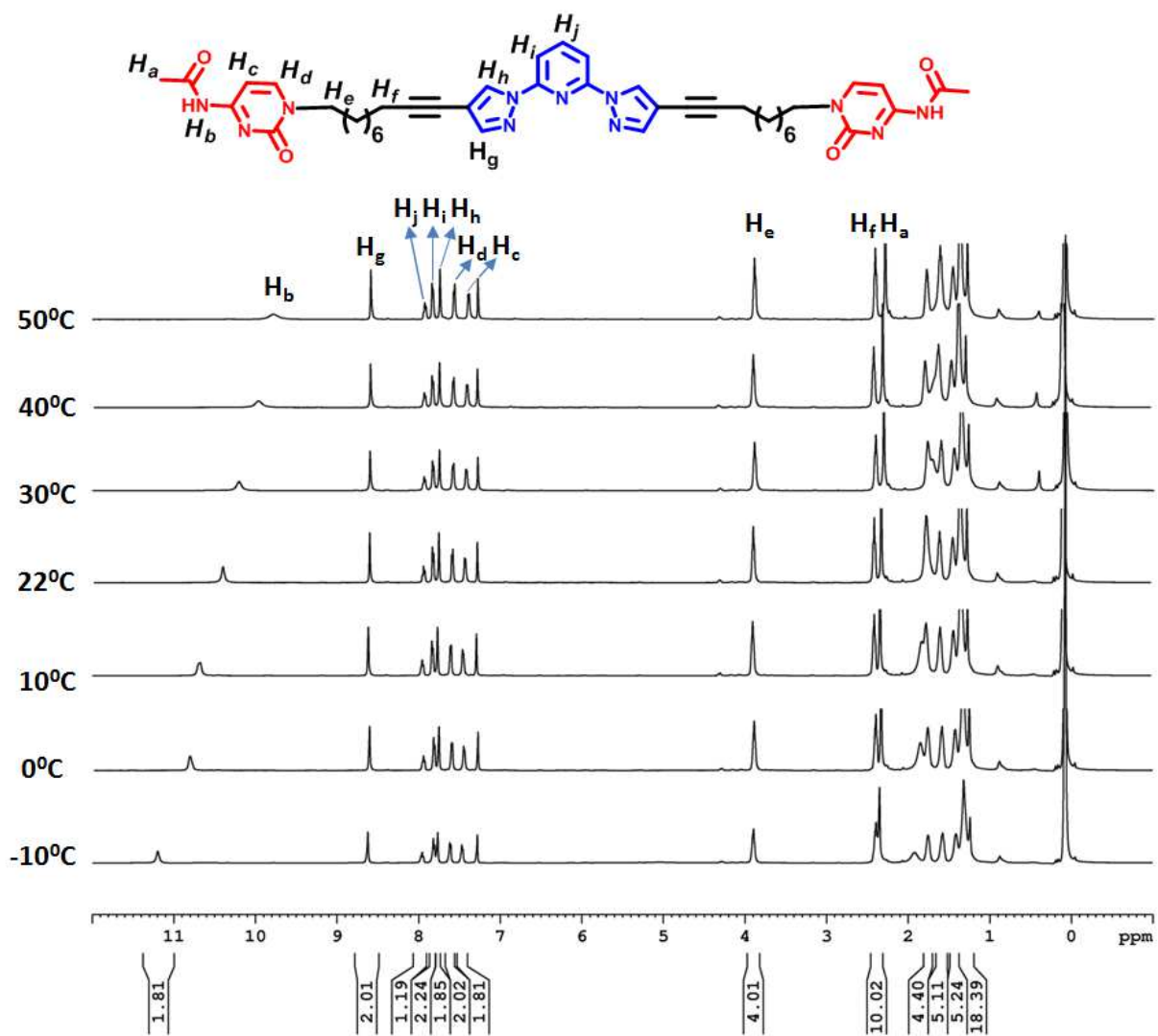
Figure S1 | Variable temperature ^1\text{H-NMR} studies of 1 in \text{CDCl}_3 .
