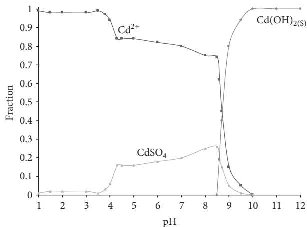
FIGURE 3: Specification diagram for \text{Cd(OH)}_2(\text{c}) by Medusa-Hydra chemical program.
