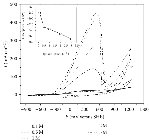
FIGURE 8: Cyclic voltammograms for methanol oxidation in 1.0 M methanol at various NaOH concentrations on Pt-Pd/C catalyst at 25°C and sweep rate of 50 \text{mV s}^{-1} ; inset: variation of onset potentials for methanol oxidation with NaOH concentration in 1.0 M methanol.
