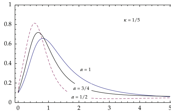
Figure 2: Approximate curves of fractional-order integrodifferential equation t versus v .
