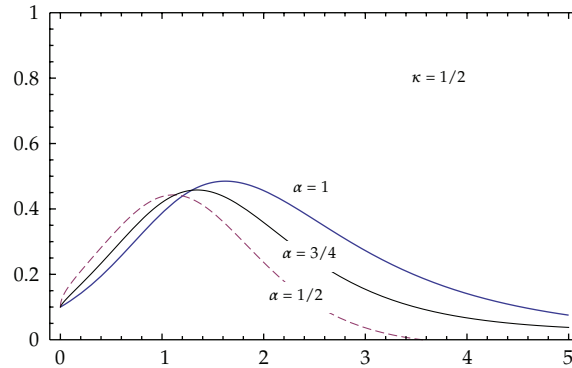
Figure 1: Approximate curves of fractional-order integrodifferential equation t versus v .
