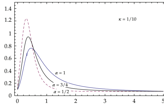
Figure 3: Approximate curves of fractional-order integrodifferential equation t versus v .
