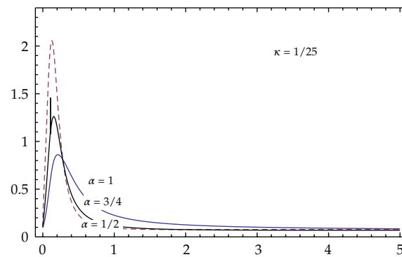
Figure 4: Approximate curves of fractional-order integrodifferential equation t versus v .
