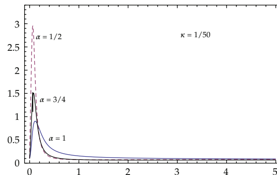
Figure 5: Approximate curves of fractional-order integrodifferential equation t versus v .
