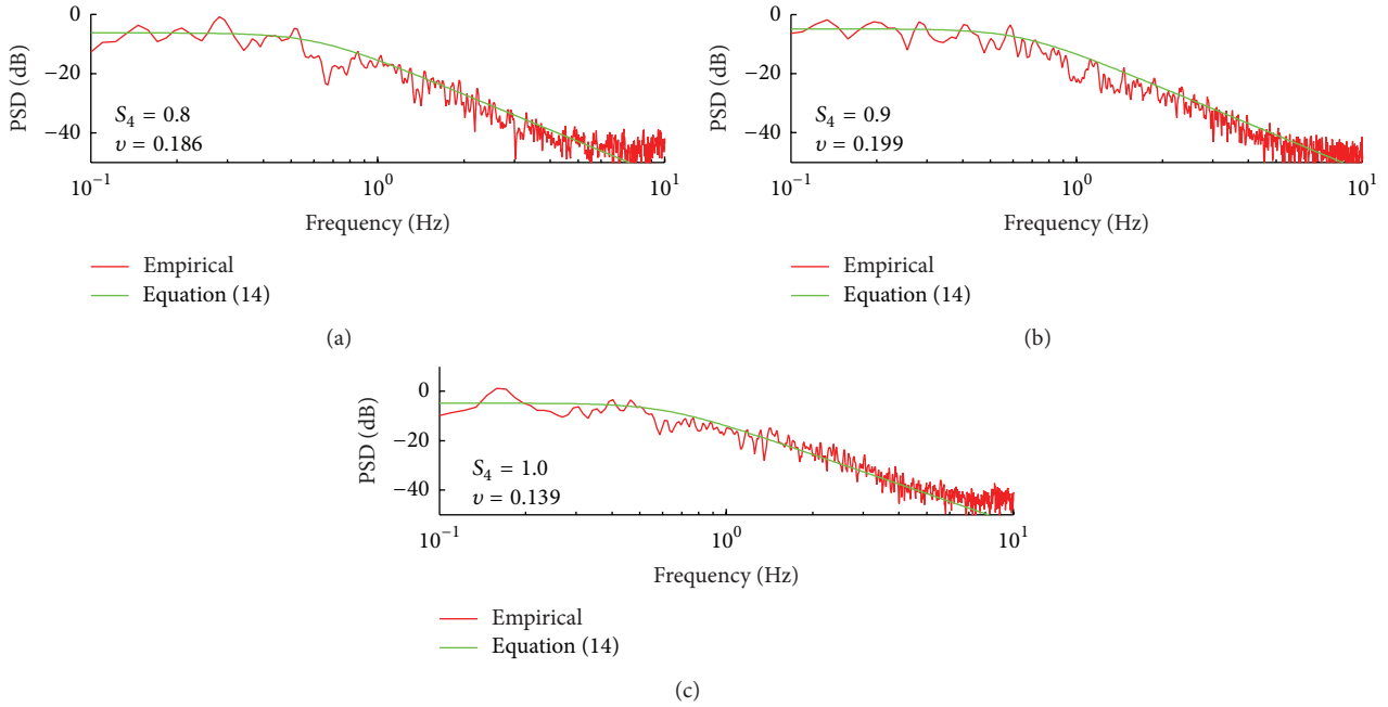
FIGURE 5: Estimated scintillation power spectral densities (red) and corresponding results (green) from the theoretical \alpha - \mu formulation represented by (14) for different values of the scintillation index S_4 .
