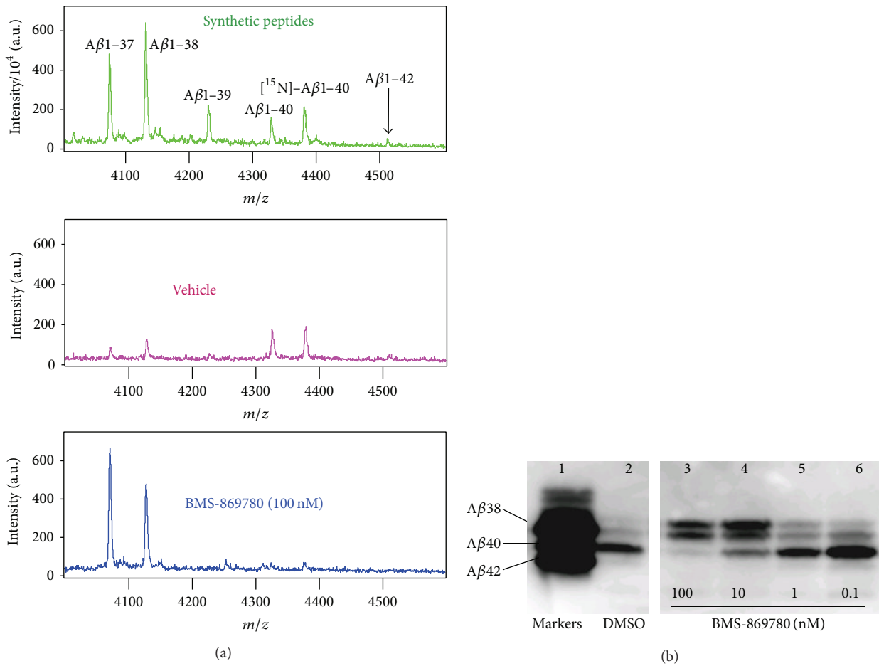
FIGURE 3: BMS-869780 increased the levels of the shorter peptides Aβ1-38 and Aβ1-37. (a) Top panel: an equimolar mix of synthetic peptides Aβ1-37, Aβ1-38, Aβ1-39, Aβ1-40, [15N]-Aβ1-40, and Aβ1-42 was evaluated by MALDI-TOF mass spectrometry. H4-APPsw cell cultures were treated with vehicle (0.1% DMSO—middle panel) or BMS-869780 (100 nM—bottom panel), [15N]-Aβ1-40 was added, and Aβ peptides were immunoprecipitated and evaluated by MALDI-TOF mass spectrometry. (b) H4-APPsw cell cultures were treated with BMS-869780 or DMSO vehicle. Aβ peptides were separated by gel electrophoresis in the presence of urea and detected by western blotting. Under these conditions, higher molecular weight Aβ peptides exhibit greater gel mobility. Lane 1: an equimolar mix of synthetic peptides Aβ1-38, Aβ1-40, and Aβ1-42. Lane 2: DMSO vehicle-treated cell culture. Lanes 3–6: Cell cultures treated with BMS-869780 at final concentrations of 100, 10, 1 and 0.1 nM, respectively.
