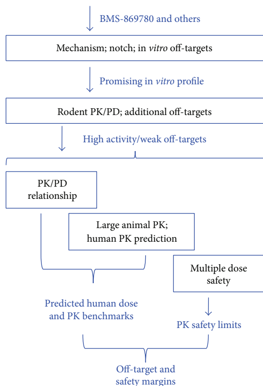
FIGURE 11: An overview of the characterization of BMS-869780 illustrates only the key steps in integration of data. Additional off-target and pharmaceuticals evaluations necessary for decisions on individual compounds are not represented in this diagram.
