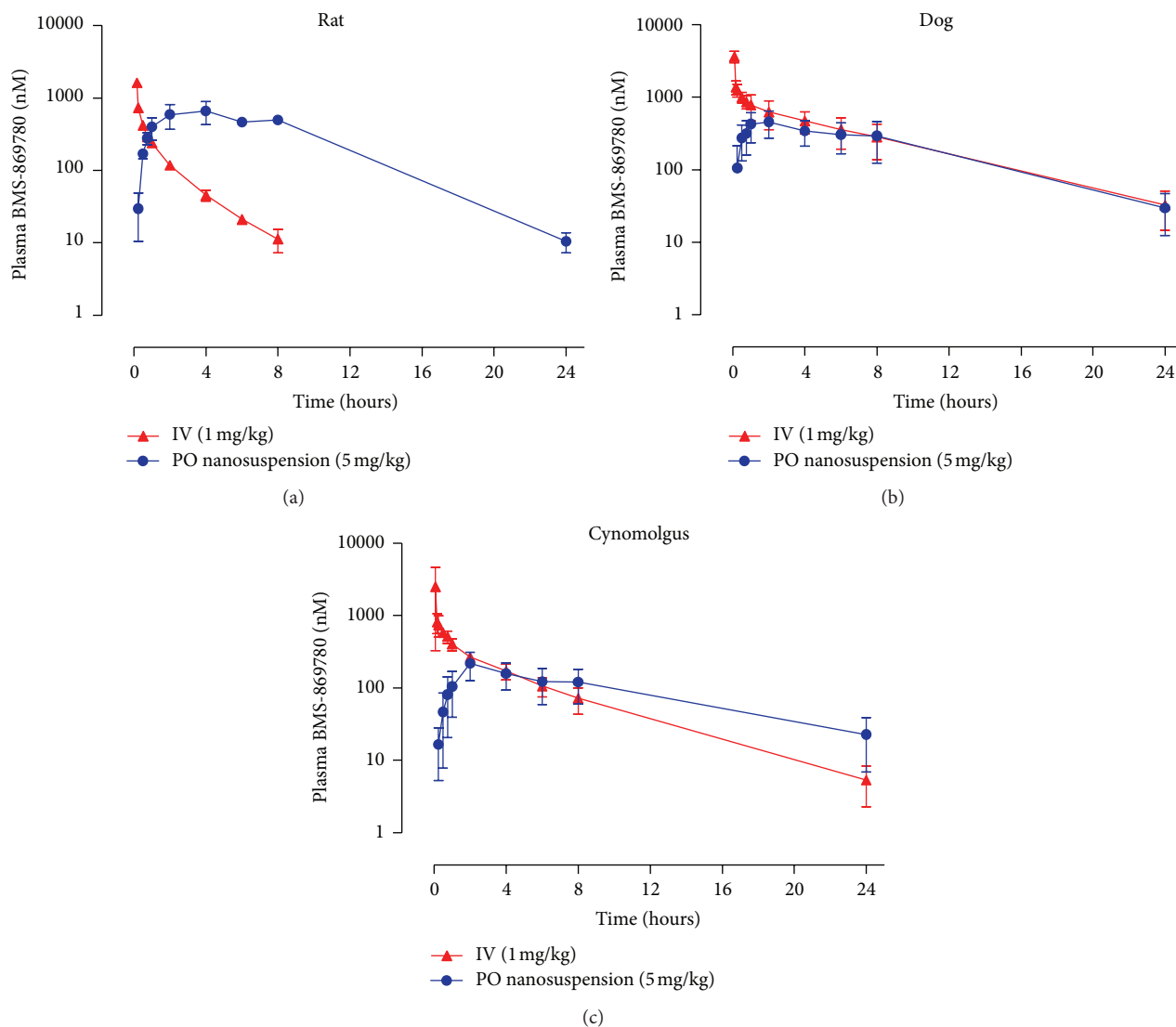
FIGURE 9: Pharmacokinetics (PK) of BMS-869780 across species for prediction of human PK. Rats, dogs, and cynomolgus monkeys were dosed with BMS-869780 intravenously (IV ▲) at 1 mg/kg or oral nanosuspension (PO ●) at 5 mg/kg. Plasma concentrations of BMS-869780 were determined for up to 24 hours after the dose. (a) Rat. (b) Dog. (c) Cynomolgus monkey. The derived PK parameters are summarized in Table 4.
