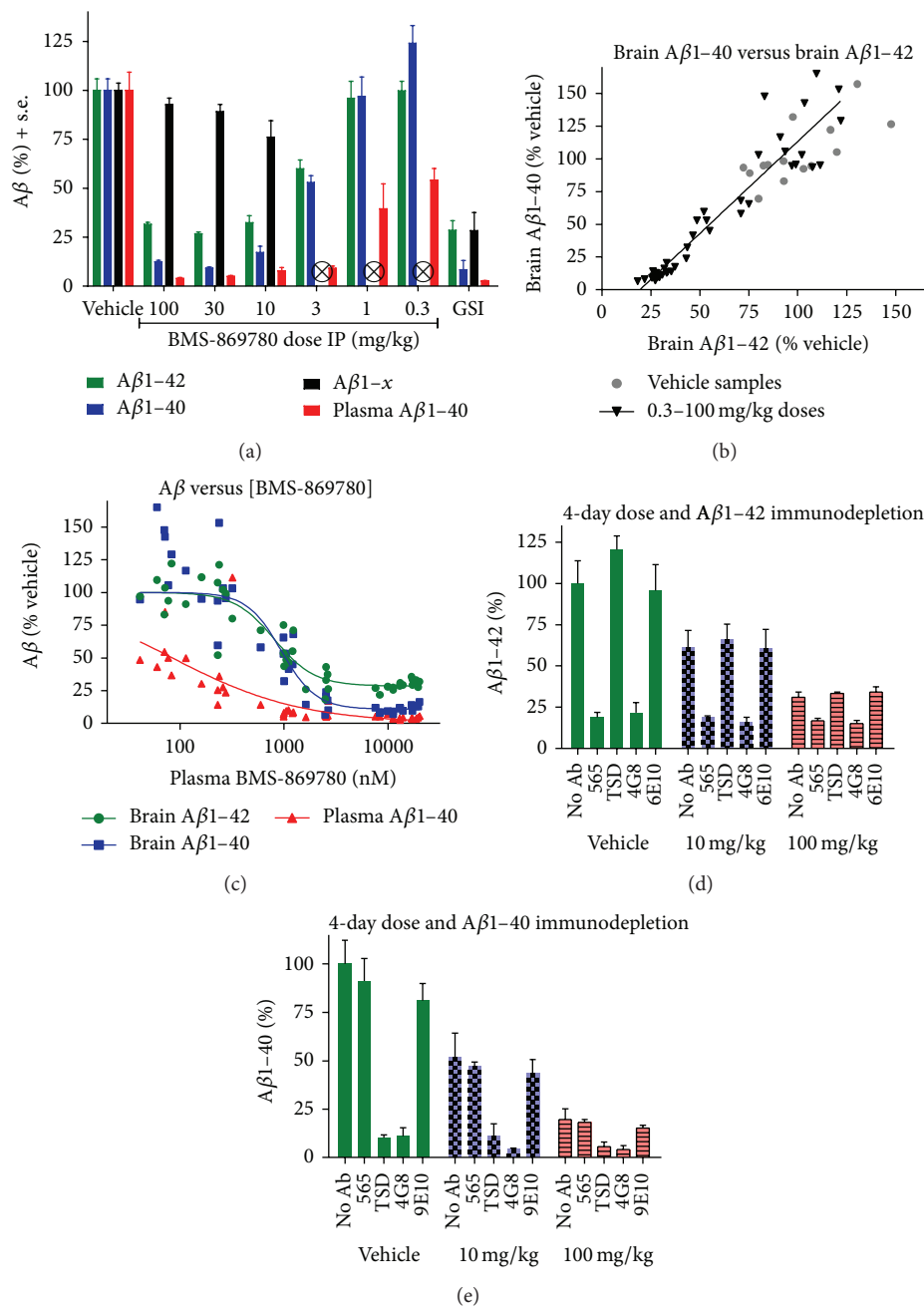
FIGURE 7: BMS-869780 dose response and evaluation of residual A\beta levels in rat brain. (a) Groups of rats received intraperitoneal (IP) injections of vehicle or BMS-869780 at doses of 100, 30, 10, 3, 1, and 0.3 mg/kg. Additional rats were dosed with GSI BMS-698861 at 30 mg/kg as a positive control for A\beta -lowering. Group sizes were seven rats for each dose of BMS-869780 and 14 rats for vehicle and GSI dose groups. Brain and plasma were harvested 5 hours after dosing. Brain A\beta 1-42 (green), brain A\beta 1-40 (blue), brain A\beta 1-x (black), and plasma A\beta 1-40 (red) were determined. Values are expressed as % relative to vehicle group mean. Whiskers represent standard error. \otimes A\beta 1-x was not determined in the groups dosed at 3, 1, and 0.3 mg/kg. (b) Brain A\beta 1-40 was plotted against brain A\beta 1-42 for each rat dosed with BMS-869780 (black \blacktriangledown ) and for each rat dosed with vehicle (grey \bullet ). Values are expressed as % relative to vehicle group mean. Whiskers represent standard error. (c) Brain A\beta 1-42 ( \bullet ), brain A\beta 1-40 ( \blacksquare ), and plasma A\beta 1-40 ( \blacktriangle ) were plotted against plasma concentration of BMS-869780 and the data were evaluated by fit to a four-parameter dose response curve. The top of the dose response curve was defined by vehicle group mean (100%), and the apparent IC_{50} values in terms of the plasma BMS-869780 concentration obtained for brain A\beta 1-42, brain A\beta 1-40, and plasma A\beta 1-40 were 807 nM, 943 nM, and 84 nM, respectively. The respective 95% confidence intervals were 618–1053 nM, 704–1264 nM, and 44–158 nM. (d) Rats were dosed once daily with BMS-869780 for 4 days at 10 and 100 mg/kg or vehicle, plasma, and brain samples were taken 5 hours after the last dose, and immunodepletion of brain extracts was carried out prior to A\beta 1-42 ELISA assays. Specific monoclonals used were 565 ( A\beta 1-42 selective), TSD ( A\beta 1-40 selective), 4G8 (binds both A\beta 1-42 and A\beta 1-40), and 6E10 (does not bind rat A\beta ). After immunodepletion, A\beta 1-42 was assayed by ELISA. (e) Same as described in (d), except that A\beta 1-40 ELISA was carried out following the immunodepletion.
