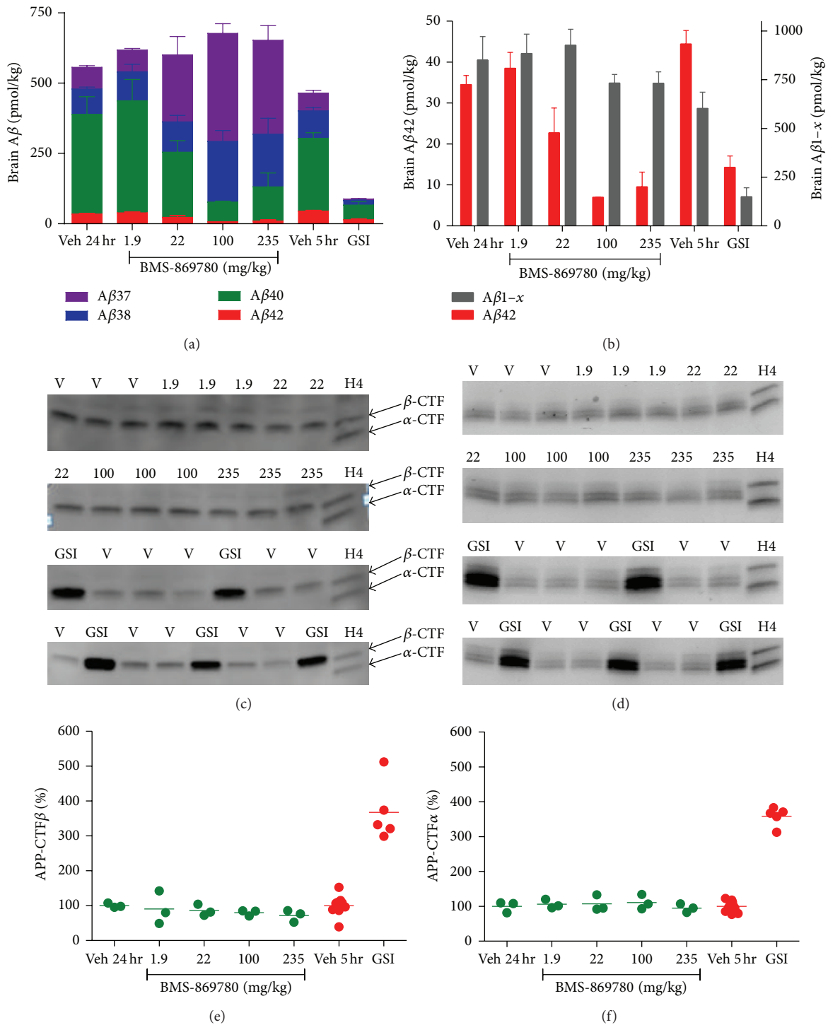
FIGURE 5: BMS-869780 modulated Aβ but did not cause accumulation of βCTF or αCTF in rat brain. Rats were given oral doses of BMS-869780, and levels of brain Aβ, βCTF, and αCTF were determined 24 hours later. For comparison, BMS-698861 was dosed in a separate experiment and samples were taken 5 hours later. (a) Brain levels of Aβ1-42 (red), Aβ1-40 (green), Aβ1-38 (blue), and Aβ1-37 (purple) are shown as bars stacked upon one another. The total height of each bar therefore represents the sum of the four peptides. (b) Aβ1-42 (red—left Y axis) and Aβ1-x (grey—right Y axis). The same results for Aβ1-42 are plotted in both (a) and (b). (c) Rat brain βCTF was detected by western blotting of immunoprecipitates from samples of the same rat brains used for Aβ determinations. V, vehicle groups; results from rats dosed with 1.9, 22, 100, and 235 mg/kg of BMS-869780 and 10 mg/kg BMS-698861 (GSI) are indicated. (d) Western blots of immunoprecipitated αCTF from the same rat brain samples. (e) and (f) quantification of western blots shown in (c) and (d), respectively, expressed relative to percent of average level of CTF in vehicle-treated rats. Actual doses of BMS-869780 were determined by analysis of concentrations in left-over dosing solutions.
