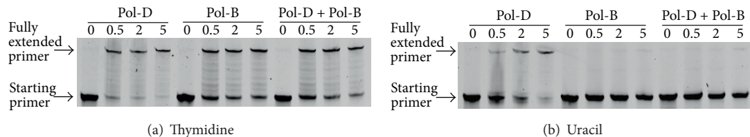
FIGURE 3: Inhibition of DNA polymerase-D by DNA polymerase-B in the presence of template strand uracil. (a) Extension of a thymidine-containing (control) primer-temple by Pol-D, Pol-B, and a mixture of Pol-D and Pol-B. (b) Extension of a uracil-containing primer-temple by Pol-D, Pol-B, and a mixture of Pol-D and Pol-B. The numbers above the gel represent the extension time in minutes. In these experiments wild type ( exo^+ ) Pol-D and Pol-B were used. These experiments were carried out three times and in every case complete inhibition of Pol-D by Pol-B was noticed when uracil was present in the template.
