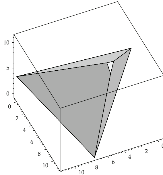
Figure 2: An example of the polytope T_4 in the case r = 4 . The vertices are in (-1/2, r - 1/2, 2r - 1/2) , (r-2/3, 2r-2/3, 3r-2/3) , (r, 2r-1, 3r-1) , (r, 2r, 3r-2) , (2r-1/2, 3r-1/2, -1/2) , and (3r-1/2, -1/2, r-1/2) .
