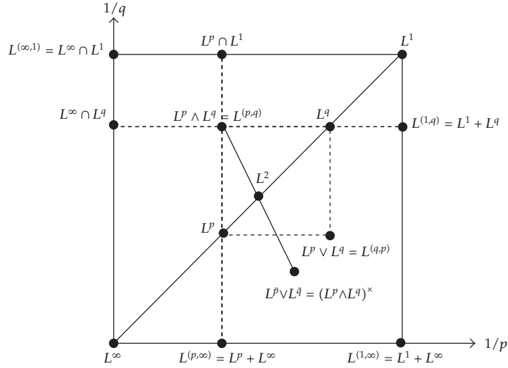
Figure 1: The unit square describing the lattice J.
