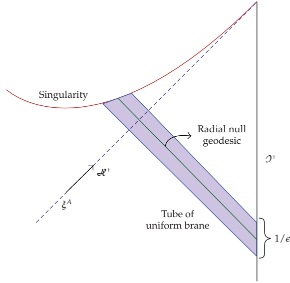
Figure 4: The causal structure of the spacetimes dual to fluid mechanics illustrating the tube structure. The dashed line denotes the future event horizon \mathcal{H}^+ generated by \xi^A , while the shaded tube indicates the region of spacetime over which the solution is well approximated by a tube of the uniform black brane.
