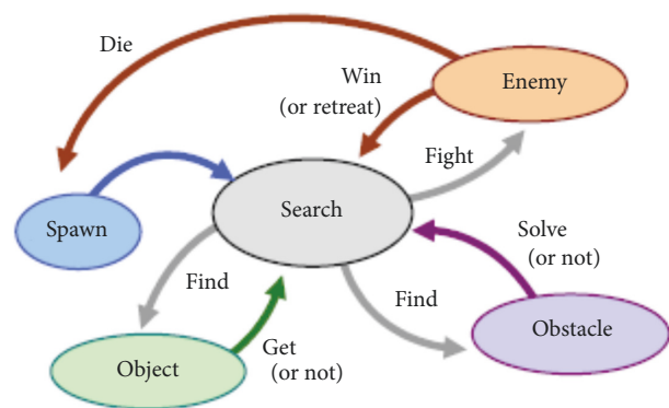
FIGURE 7: A simple FPS game state transition illustration.
